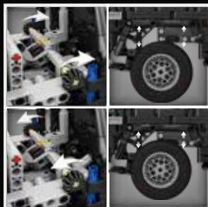
硬度可调节避震 adjustable stiffness suspensions
